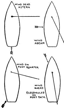
Diagram No. 1. Sailing under Varying Conditions of Wind.
